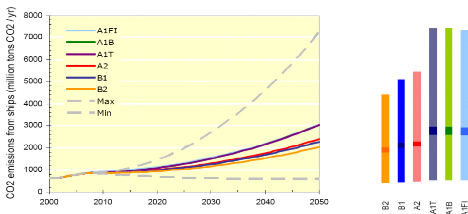
Figure 2: Projections of maritime transport CO 2 emissions
